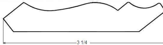
3-1/4" Crown Stocked in Red Oak
