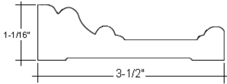
3-1/2" RB3 Stocked in MDF
