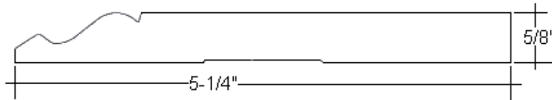
5-1/4" Speed Base Stocked in MDF, 16' lengths only
