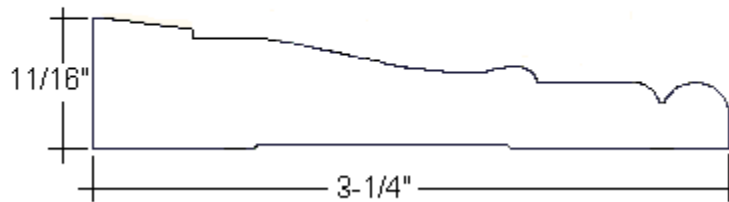
3-1/4" #445 Colonial Stocked in MDF
